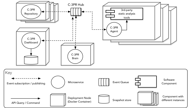
Fig. 3. C-3PR building blocks (implemented using microservices)
