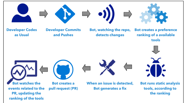
Fig. 1. C-3PR Workflow
